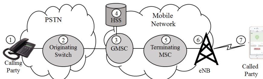
Fig. 1 Simplified PSTN-to-mobile call setup
